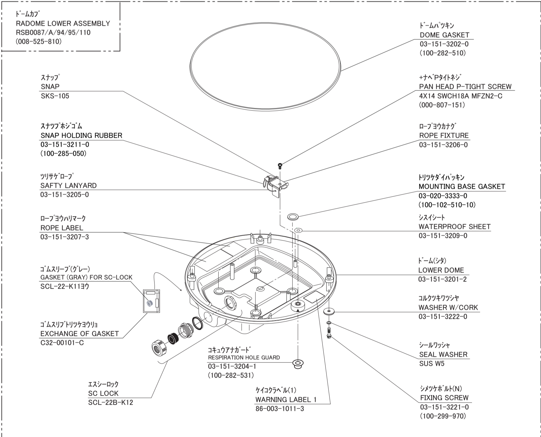
取付台組品 TRANSCEIVER UNIT W/RADIATOR
